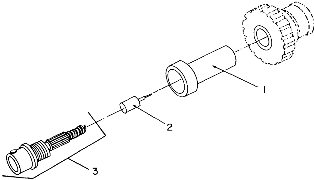
Figure 5. Probe, Waveguide MX-1546/USM-37E.
